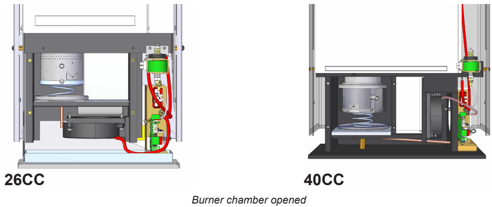
Burner chamber opened
