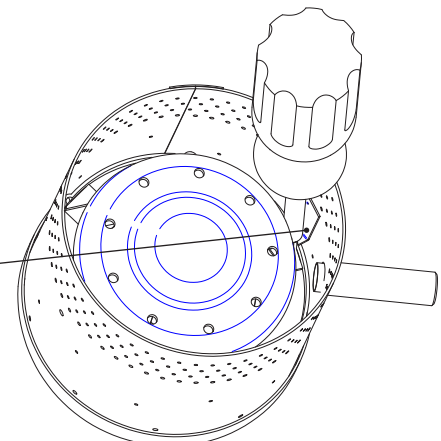
Picture 6. Detaching the radiation element
